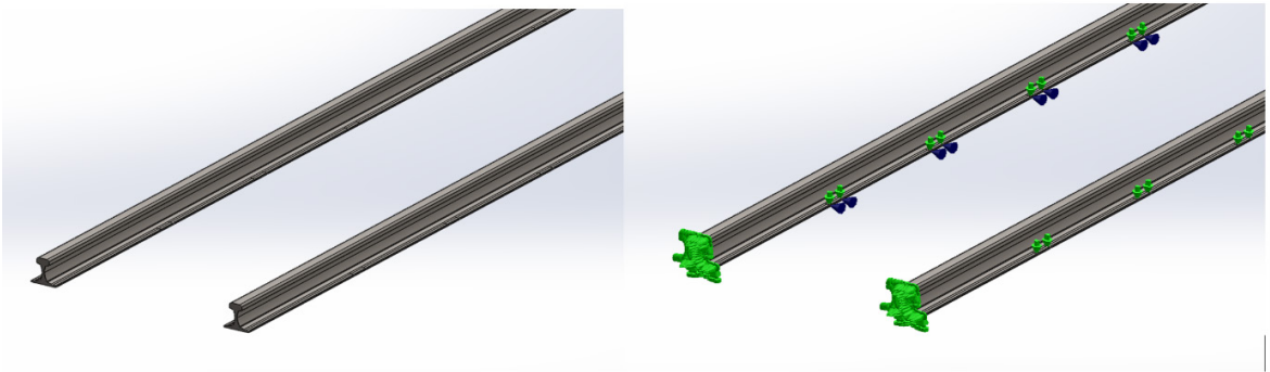
Figure 7 Railway model and fastening setup (Boundary conditions).
