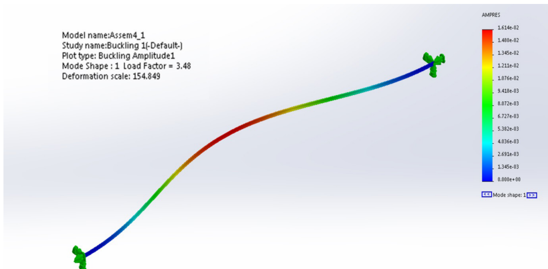
Figure 2 Buckling temperature analysis of a rail fixed at both ends.
