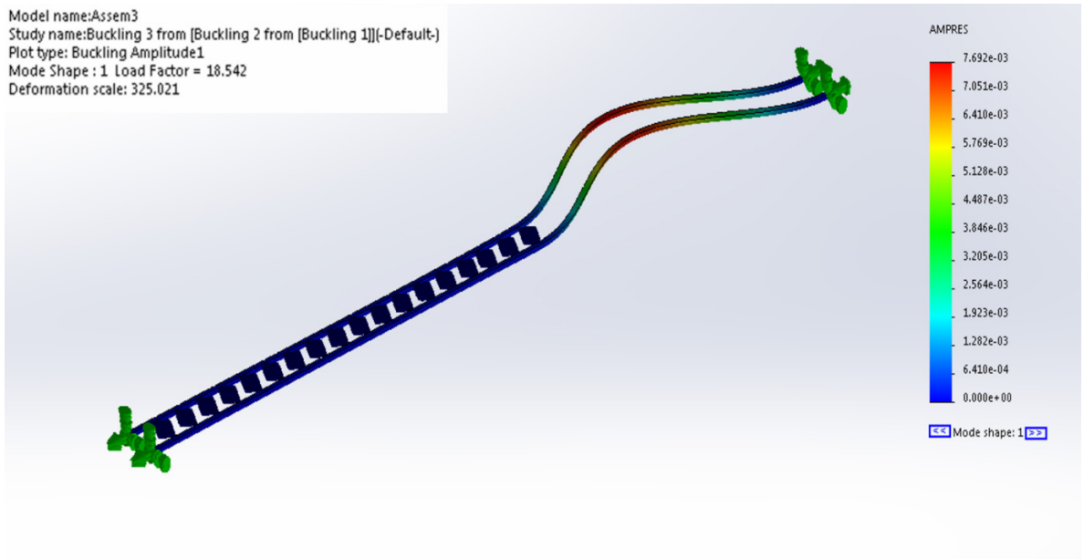
Figure 8 Lateral buckling of the railway track.
