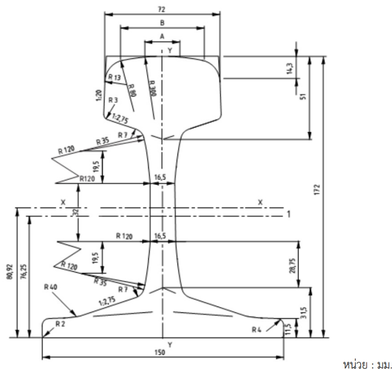
Figure 1 Rail cross-section type UIC60.
